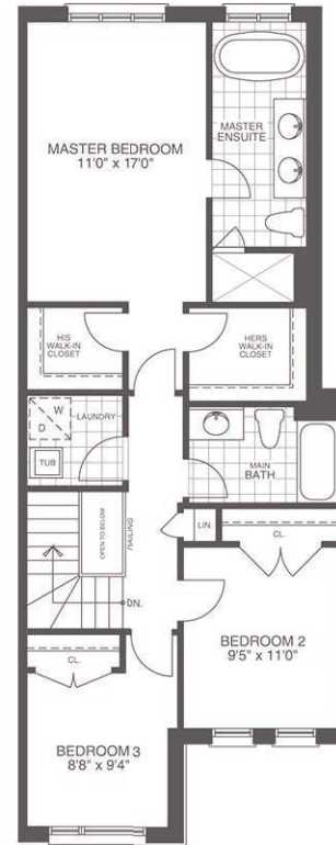
SECOND FLOOR PLAN ELEVATION A 1602 sf
